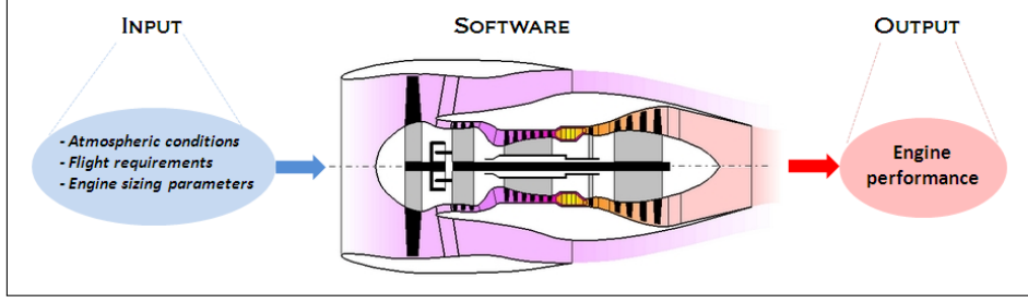
FIGURE 1. Aeronautic software
