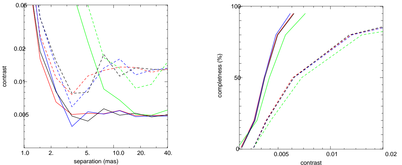
Fig. 3. Left: 3\text{-}\sigma sensitivity versus separation for a completeness level of 80%. Right: Completeness in the separation range 6 – 40 mas versus contrast. Simulations are for a single snapshot pointing (dashed lines) and for five pointings separated by one hour (solid lines). Colours are for the four configurations of VLTI displayed in Fig. 1. The contrast axes can be scaled for any given accuracy of the closure phase measurements (here \sigma = 0.25 deg).
