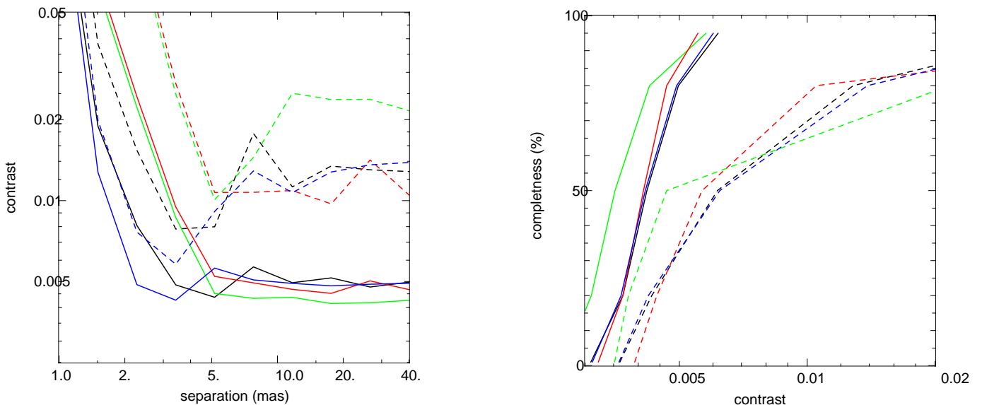
Fig. 5. Left: 3\text{-}\sigma sensitivity versus separation for a completeness level of 80%. Right: Completeness in the separation range 6 – 40 mas versus contrast. Simulations are for a single snapshot pointing (dashed lines) and for five pointing separated by one hour (solid lines). Colours are for the four configurations displayed in Fig. 4. The black curves are for the U1-U2-U3-U4 configuration displayed in Fig. 1. The contrast axes can be scaled for any accuracy on the closure phase (here \sigma = 0.25 deg).
