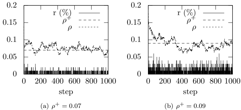
Figure 5: Simulation examples with k_P = 10 \cdot \rho^+ and initial density \rho(t_0) = 2 \cdot \rho^+ . r represents the rate of microscopic influences not taken into account (in %) by Reaction^{lm} .
