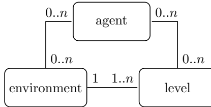
Figure 1: Main concepts of IRM4MLS (as a simplified class diagram)
