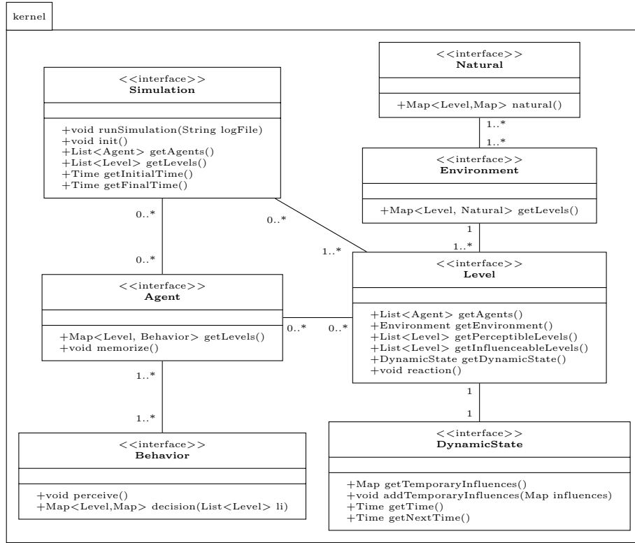
Figure 2: Java API of IRM4MLS
