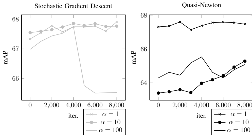
Fig. 3. Mean average precision as a function of the number of iterations for the Vehicle dataset, with SGD (left) et QN (right) optimization methods.
