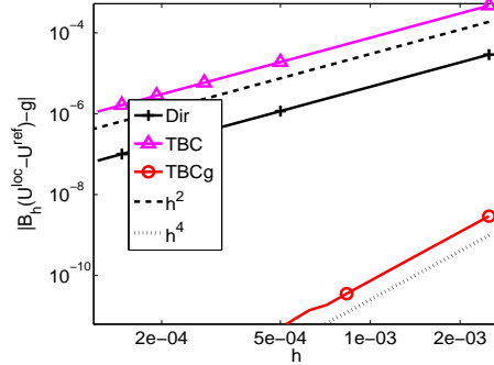
Figure 4: Residual |B_h(U^{\text{loc}} - U^{\text{ref}}) - g| at point x_{2i_0} = 0.4 as a function of h for the Dirichlet OBC (Dir), the transparent OBC with no correction term (TBC) and the generalized OBC (TBCg).
