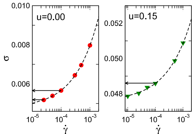
FIG. 8: Global flow curves \sigma = \sigma(\dot{\gamma}) for the repulsive particles with u = 0.0 (left) and attractive particles with u = 0.15 (right). The data are shown with symbols, while the dashed lines are fits to the Herschel-Bulkley form, Eq. (4). Horizontal arrows indicate the stress values at which constant stress simulations are performed, see Figs. 9 and 10. Notice the very different stress scales used in both panels.
