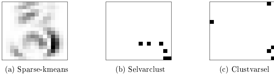
Figure 3: Variable selection obtained from (a) the sparse-kmeans algorithm, (b) the Selvarclust approach and (c) the Clustvarsel approach.
