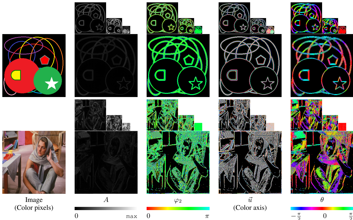
Fig. 3. Color monogenic wavelet transform on synthetic image and barbara image.
