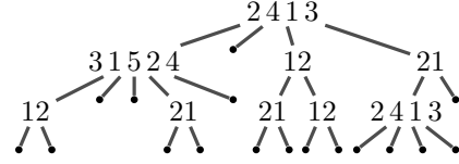
Fig. 1: Decomposition tree of \pi (from Ex. 2.2).
