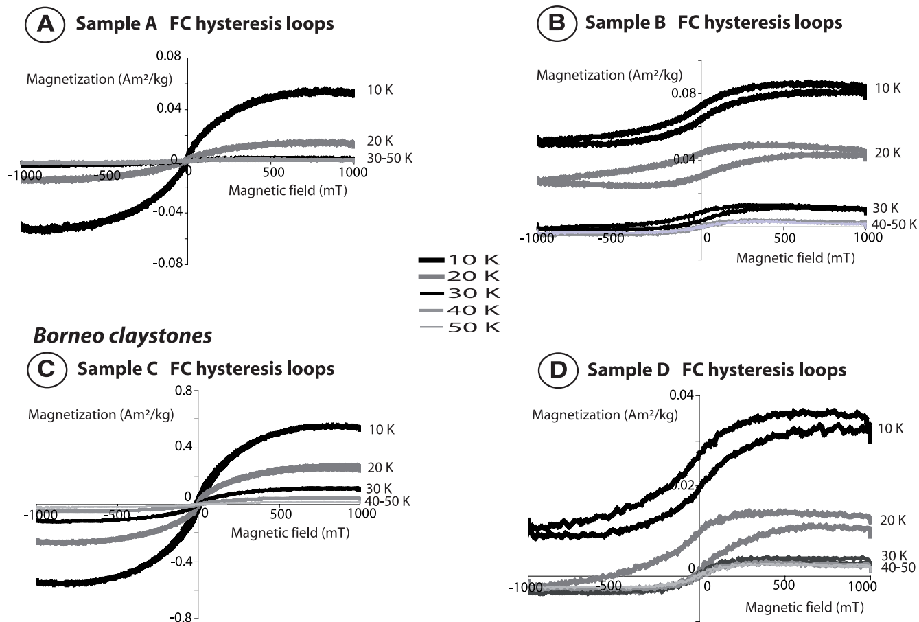
Figure 2. Field Cooled hysteresis loops from 50 K to 10 K for (a) sample A, (b) sample B from the Netherlands, and (c) sample C and (d) sample D from Borneo.
