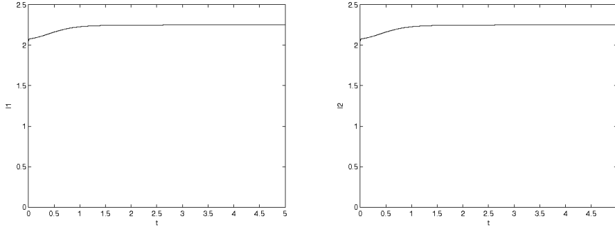
Figure 3: Dynamics of the total populations: I_\varepsilon^1(t) (left) and I_\varepsilon^2(t) (right), using the parameters in 35. In both patches, the total population converges to a constant close to 2.25.
