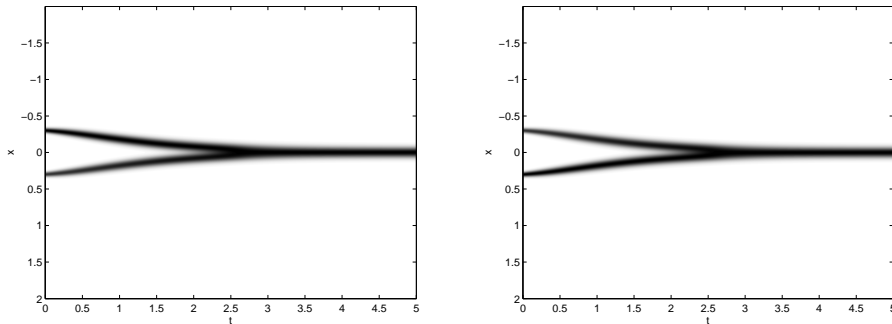
Figure 1: Dynamics of the time-dependent problem 1 with parameters given in 35 . In both figures, horizontally is time t and vertically is trait x . The gray layers represent the value of n_\varepsilon^1 (left) and n_\varepsilon^2 (right). Initially n_\varepsilon^1 is concentrated on x = -0.3 and n_\varepsilon^2 is concentrated on x = 0.3 . Due to migration both traits appear rapidly in the two patches, but in large time only one dominant trait persists. This point is the mean value of favorable traits in each patch in absence of migration.
