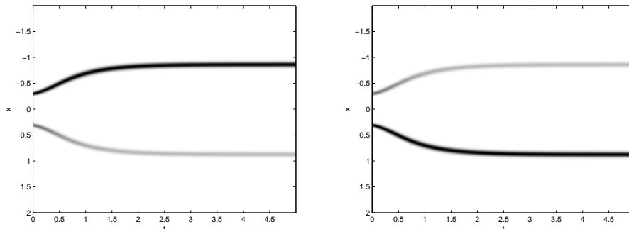
Figure 2: Dynamics of the time-dependent problem 1 with parameters given in 36 . In both figures, horizontally is time t and vertically is trait x . The gray layers represent the value of n_\varepsilon^1 (left) and n_\varepsilon^2 (right). In absence of migration, the local optimal trait in patch 1 is x = -1 and in patch 2 is x = 1 . Initially n_\varepsilon^1 is concentrated on x = -0.3 and n_\varepsilon^2 is concentrated on x = 0.3 . Due to migration both traits appear rapidly in the two patches, and evolve to two points close to -0.86 and 0.86 .
