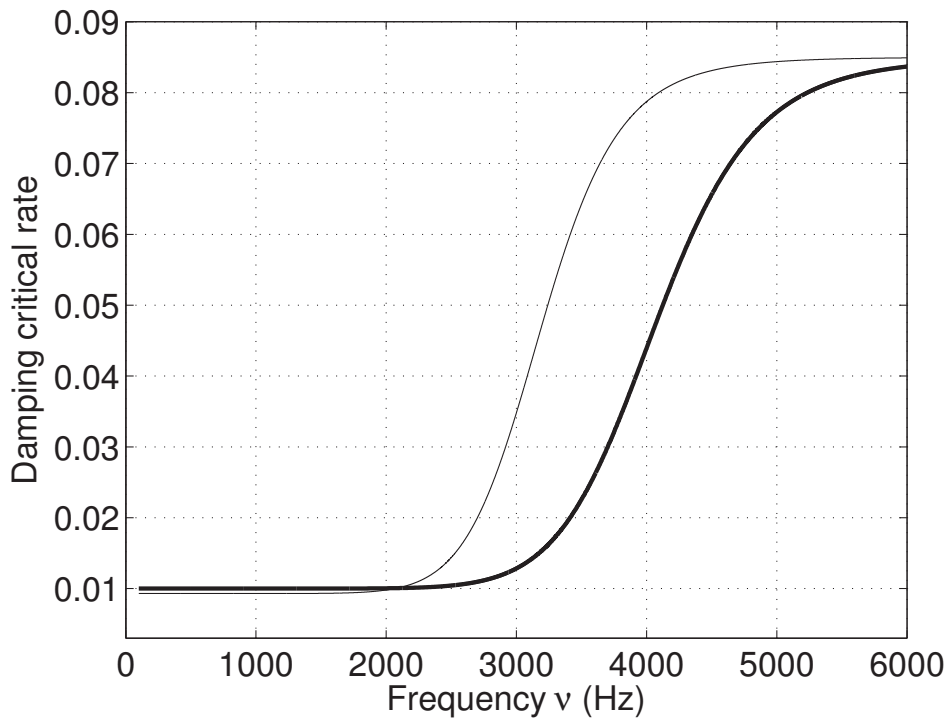
Fig. 13. Comparison between the damping model corresponding to the deterministic updating and to the robust updating. Graph of \nu \mapsto f(\nu, \mathbf{r}^0) (thick line) and \nu \mapsto f(\nu, \mathbf{r}^{RU}) (thin line).
