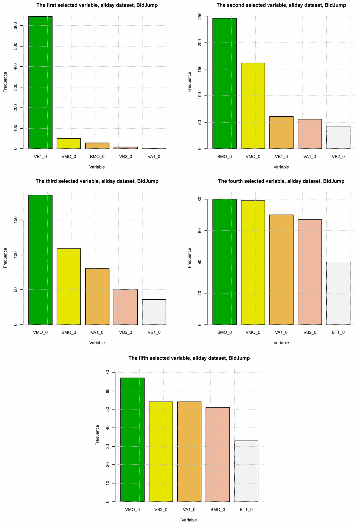
Figure 7. Variable selection for BidJump prediction, CAC40, April, 2011. From left to right, from top to bottom, each figure shows how many times a variable is selected as the k^{th} selected variable by LASSO, k = \{1, \dots, 5\} .
