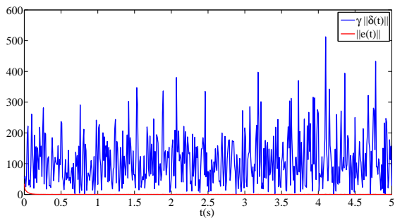
Fig. 2. Time evolution of \|e(t)\| (red) and \sqrt{7}\|\delta(t)\| (blue) with noised measurement
