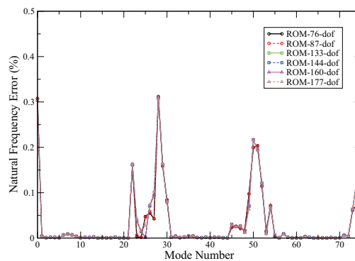
Figure 7. Comparison of the 76 first mistuned natural frequencies errors between the full model and several ROM sizes.
