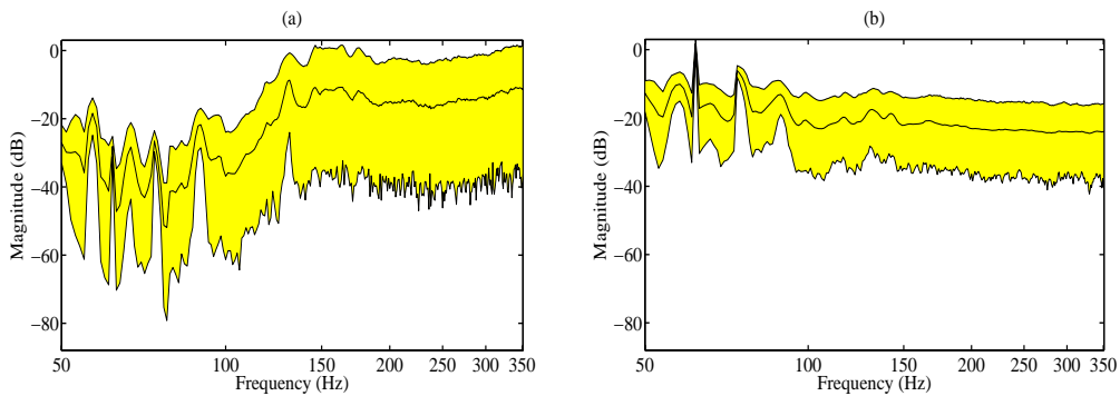
Figure 8. Confidence regions of \mathbf{T}^{loc}(\omega) (a) and \mathcal{E}^{loc}(\omega) (b). Excitation is a force applied to a given point on the structure in the X^\ell direction. Observation is the velocity in another point of the structure in the X^\ell direction. Medium line is the mean value. Upper and lower lines delimit the confidence region.
