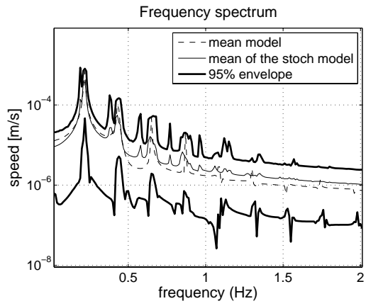
Figure 12: Stochastic response for \delta = 0.01 . ROP (a) and its frequency spectrum (b).
