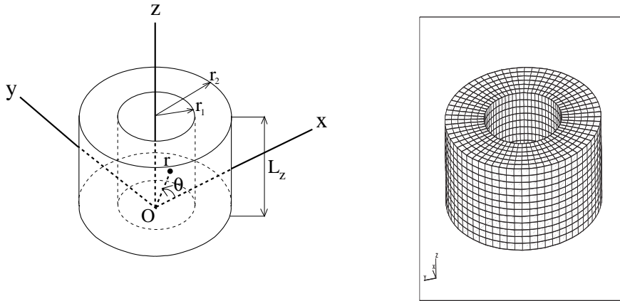
Figure 1. Geometry of the domain and coordinate systems (left figure). Finite element mesh of the domain (right figure).
