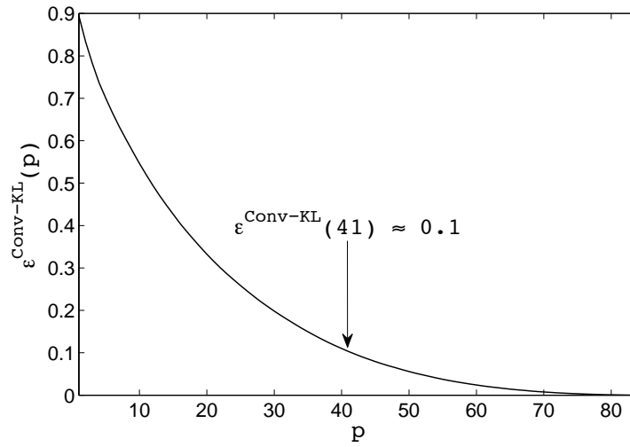
Figure 27: Graph of function p \rightarrow \epsilon^{\text{Conv-KL}}(p) .
