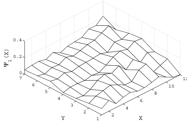
Figure 14: Graph of the first eigenfunction \mathbf{x} \rightarrow \psi_1(\mathbf{x}) .
