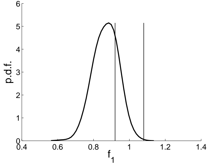
Figure 7: Probability density function of the first dimensionless eigenfrequency with (\underline{\mathbf{x}}, \delta_X) = (\underline{\mathbf{x}}^{opt}, \delta_X^{opt}) and \delta_{MK} = (0, 0) . The vertical lines delimit the [0.92, 1.08] critical range.
