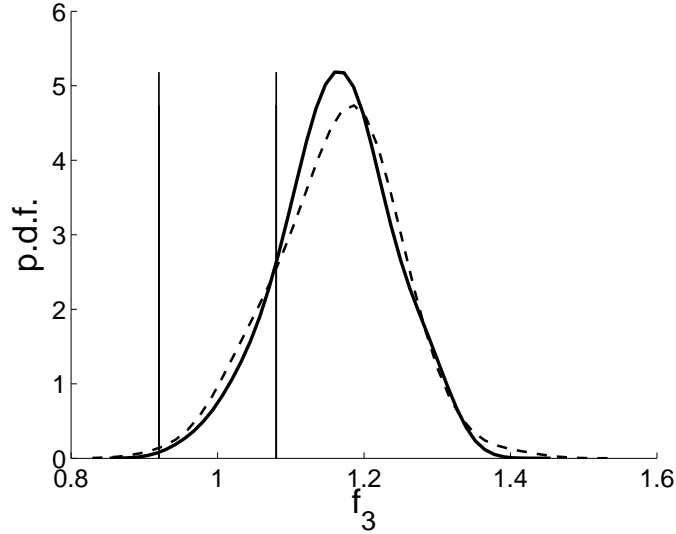
Figure 12: Probability density function of the third dimensionless eigenfrequency: with (\underline{\boldsymbol{x}}, \boldsymbol{\delta}_X) = (\underline{\boldsymbol{x}}^{opt}, \boldsymbol{\delta}_X^{opt}) and \boldsymbol{\delta}_{MK} = \boldsymbol{\delta}_{MK}^{opt} (thick solid line), with (\underline{\boldsymbol{x}}, \boldsymbol{\delta}_X) = (\underline{\boldsymbol{x}}^{opt}, \boldsymbol{\delta}_X^{opt}) and \boldsymbol{\delta}_{MK} = (0, 0) (dashed thin line). The vertical lines delimit the [0.92, 1.08] critical range.
