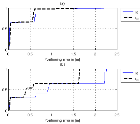
Fig. 11. Positioning error CDFs using Middle Alva antennas, after ambiguities solving, eMAL (a) and MAL (b) algorithm
