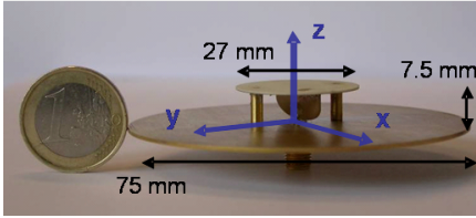
Fig. 7. Monopolar Wire-Patch (MWP) antenna
