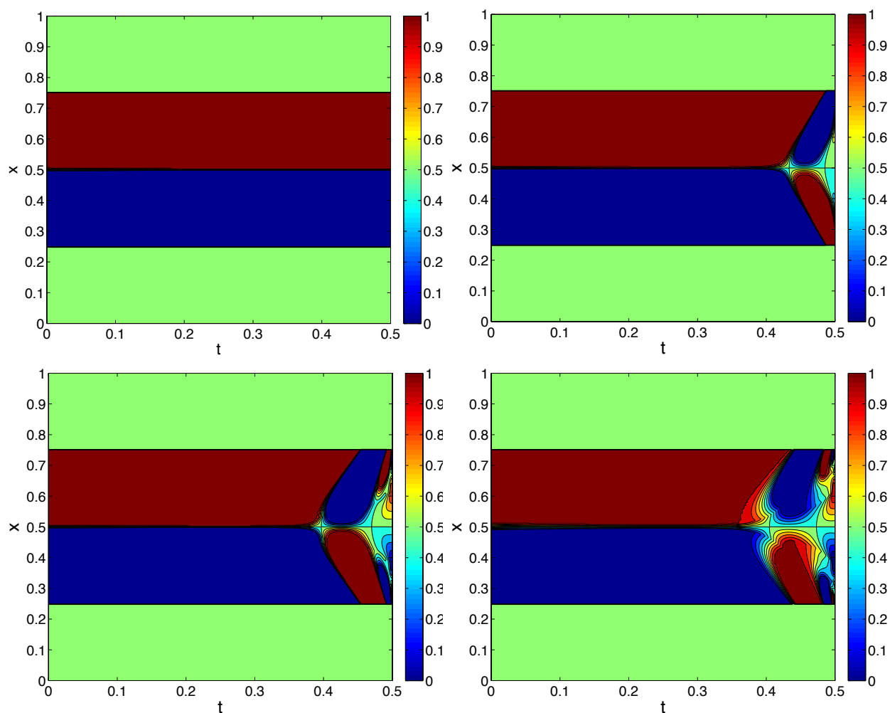
Figure 1: N_x = N_t = 400 - y_0(x) = \sin(2\pi x) - \omega = (0.25, 0.75) - c = 0.1 - From left to right and from top to bottom, iso-values of the density function s_h in Q_T for \alpha = 10^{-2}, 10^{-4}, 10^{-6} and \alpha = 10^{-8} .
