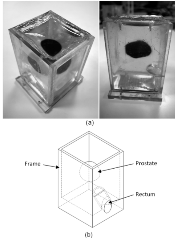
FIG. 1. (a) Photograph of the phantom with mobile prostate and rectum. (b) CAD drawing of phantom. Note that the rectum shown in this figure is meant for an end-fire US probe. For side-fire probes, a cylindrical rectum is used, as shown in Figure 11.
