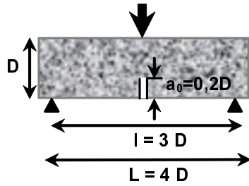
Figure 1. Geometry of the specimens.
