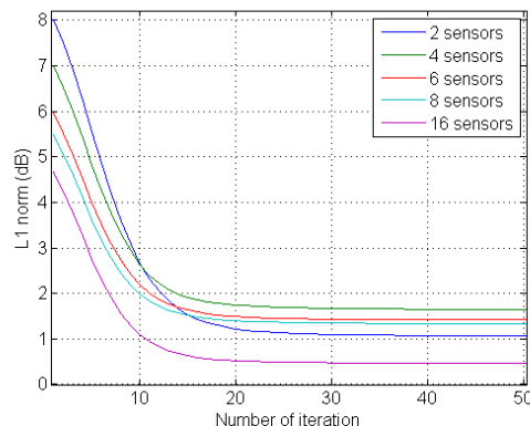
Fig. 8: The mean of the l_1 norm through the iteration of the BSS algorithm
