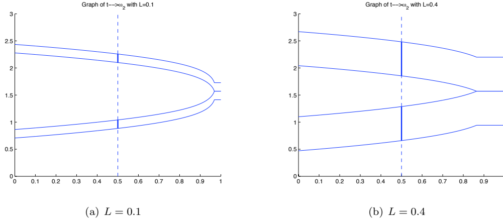
Figure 2: Optimal domain \omega^2 in function of t
