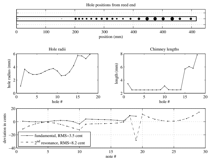
Figure 5: Design (a), corresponding to a clarinet with no dedicated register hole. The upper part of the figure shows the positions of the 18 tone holes; the two last holes on the right correspond to the acoustical lattice replacing the bell, and have not been optimized (see § 2.4). The two intermediate figures give more detail on the geometry of these tone holes. The lowest part of the figure shows the difference between the position of the impedance resonances and those of a perfect chromatic scale with equal temperament. Notes 1–19 are the first (lower) register notes, notes 20–29 are second register notes calculated from the second resonance of the impedance. One notices the particular position of the first hole, which is unusually separated from all the others; this is a consequence of its dual acoustical role (register and tone hole).
