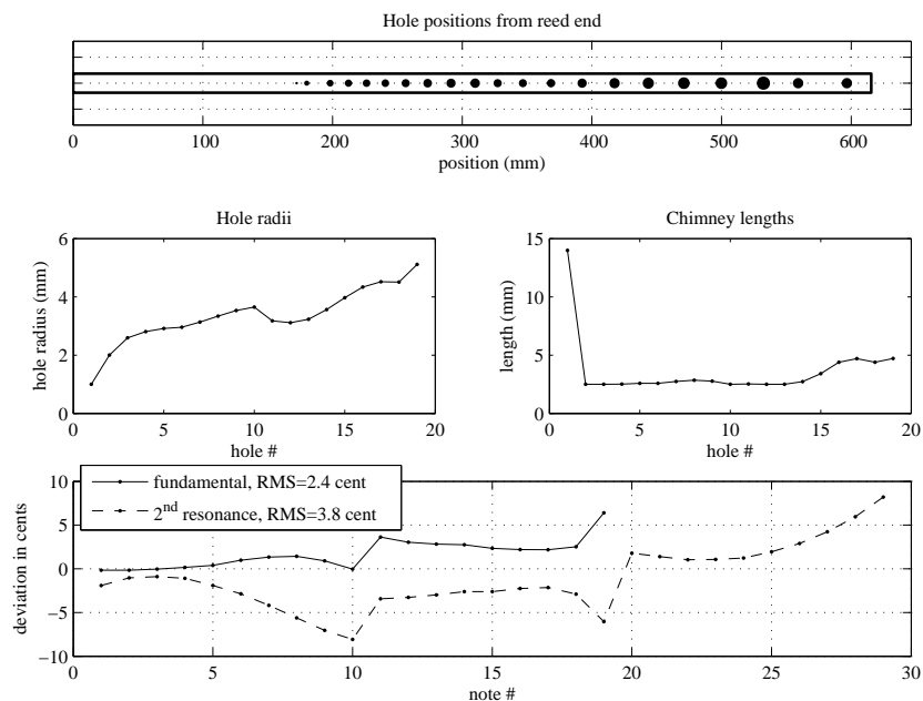
Figure 7: Design (c) with a specific register hole, but no bore enlargement. The different parts of the figure are defined as explained in the caption of Fig. 5. Here, the length of the register hole, about 15 mm, is comparable to that of real clarinets.
