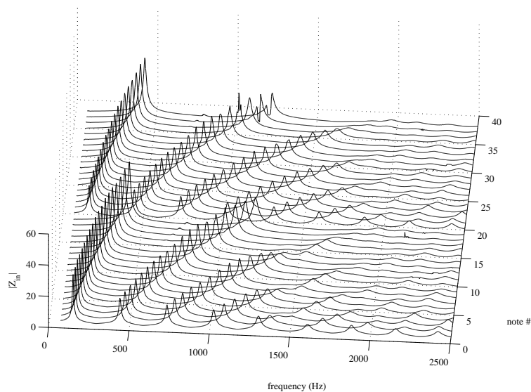
Figure 18: Measured input impedance spectrum of the experimental clarinet. This figure shows good agreement with the computed results of Fig. 11.
