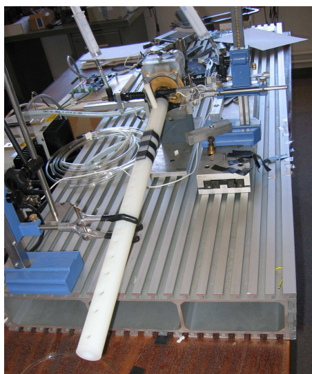
Figure 14: The prototype instrument attached to the artificial mouth.
