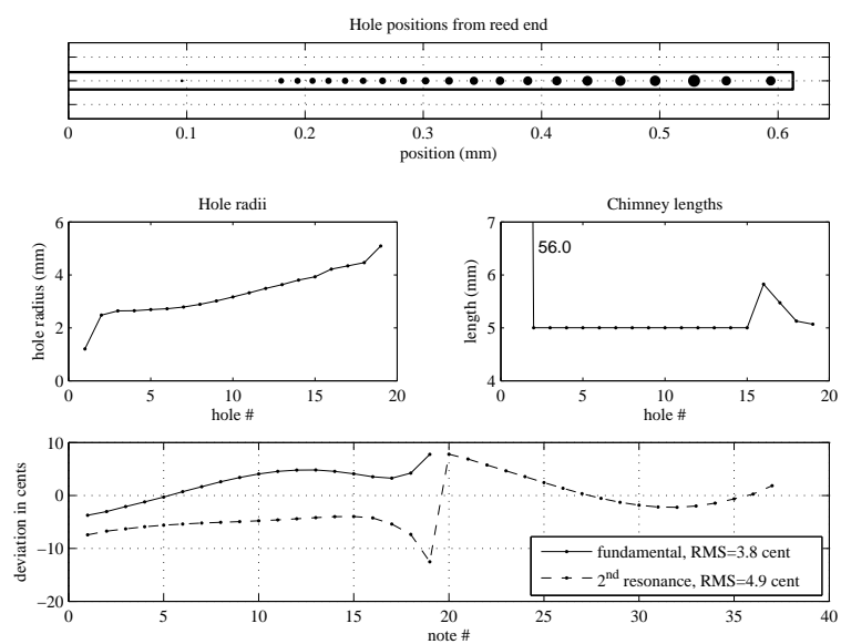
Figure 10: Design (e) of an instrument where the same number of resonances would be aligned for both registers, including the upper notes of the second register. The different parts of the figure are defined as explained in the caption of Fig 5. The register hole in this case turns out to be rather long, namely 56 mm.
