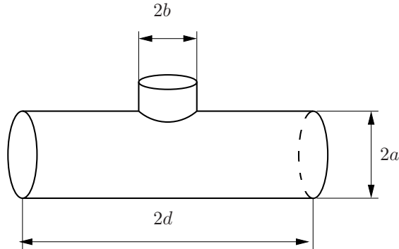
Figure 1: Elementary cell with tone hole.
