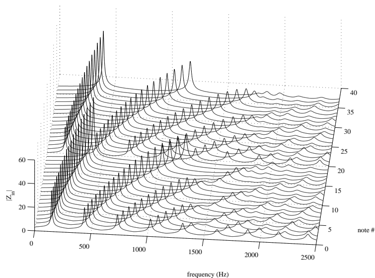
Figure 11: Computed input impedance spectra for the 37 notes of design (e). The impedance is made dimensionless by dividing it by the characteristic impedance Z_0 defined in § 2.2. The impedance peaks are similar to those of a real clarinet but, for the second register, the second peak remains smaller than the first one, because of the long register hole.
