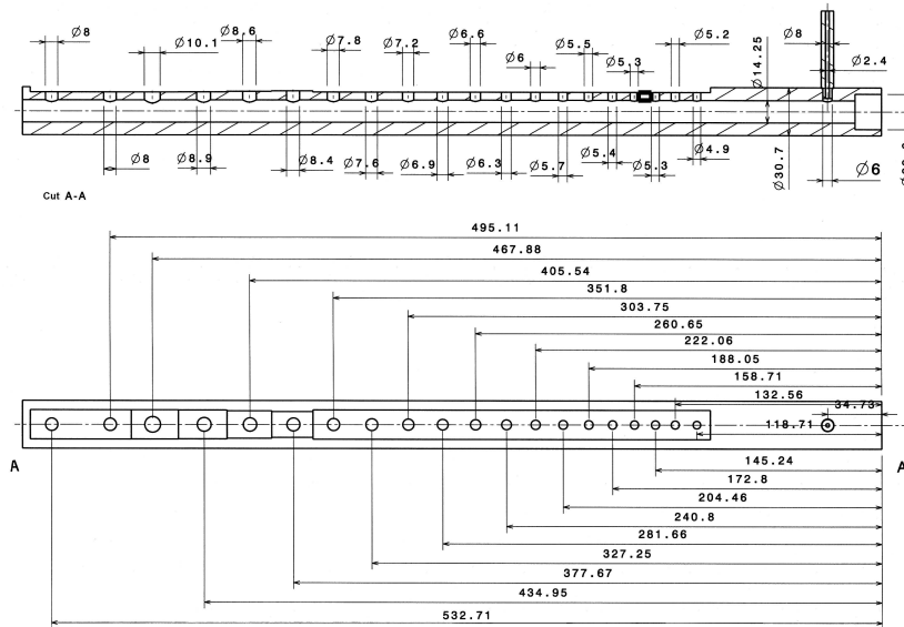
Figure 19: Drawing of the prototype instrument.
