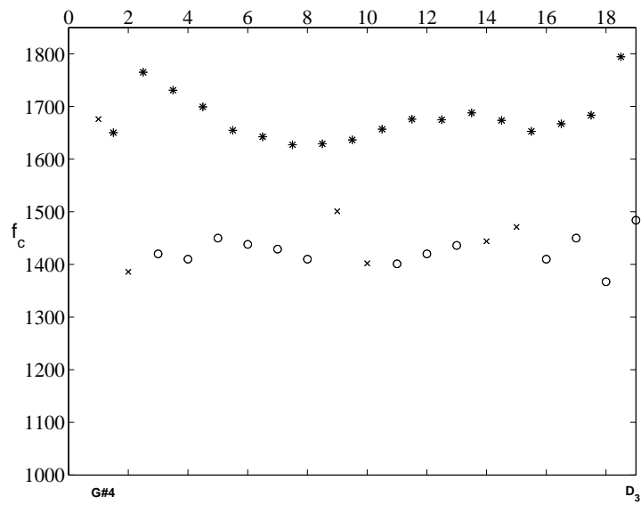
Figure 12: The local cutoff frequencies for a set of two holes are shown with stars (*). A star located at n + 1/2 corresponds to the cutoff frequency of the set of two holes (n, n + 1) . The star located at 18.5 is calculated for the hole 18 and the first vent-hole. The circles and crosses represent the global cutoff frequencies obtained in § 6 from the measurement of the input impedance, for the notes of the first register from D3 to G#4. Circles correspond to well defined values, crosses to more uncertain values.
