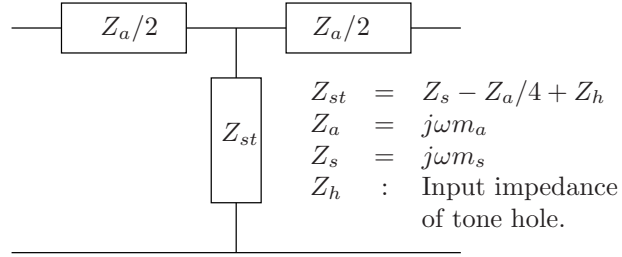
Figure 2: T-circuit equivalent for a tone hole.
