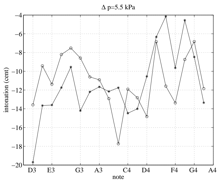
Figure 17: The experimental clarinet: measured intonation errors with a blowing pressure of 5.5 kPa (two realizations).
