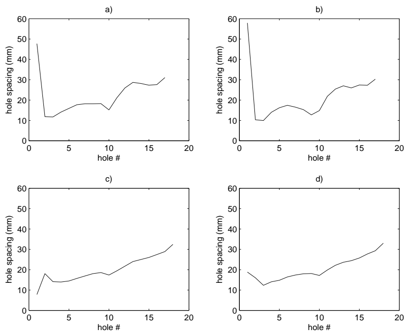
Figure 13: Distances between adjacent tone holes for instruments (a)–(d).
