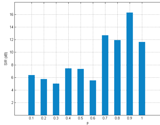
Figure 11: SIR for SP6 in the first position ( 0^\circ/30^\circ ) with p varying from 0.1 to 1 (same p through the iterations)
