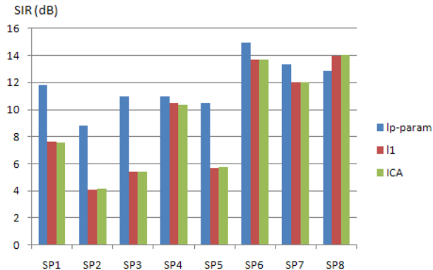
Figure 7: SIR of the blind source separation algorithms for the first position 0^\circ/90^\circ ( SP_i refers to the i th Source Pair)
