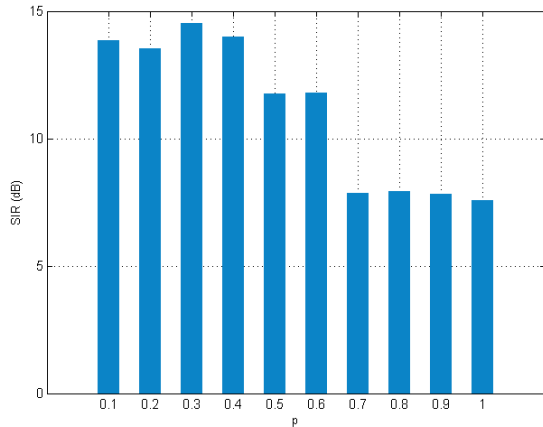
Figure 10: SIR for SP1 in the first position ( 0^\circ/90^\circ ) with p varying from 0.1 to 1 (same p through the iterations)
