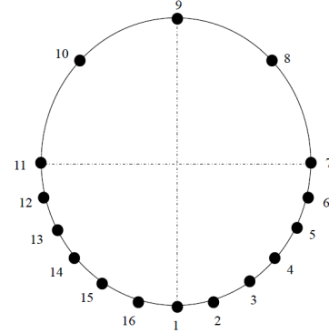
Figure 5: The geometry of the microphone array
