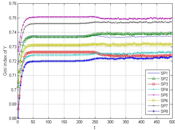
Figure 9: The Gini index of the estimated sources through the iterations in the first recording situation
