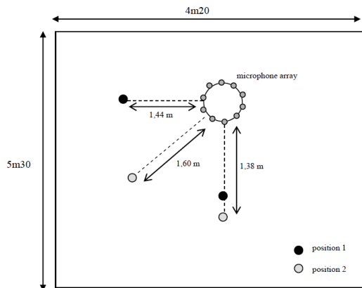
Figure 6: The position of the sound sources and the microphone array in the reverberant room
