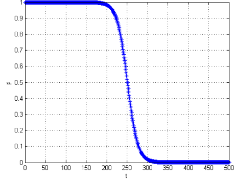
Figure 2: The parameter p as a logistic function, p = p(t) = \frac{1}{1 - \exp(-L + \frac{(t-1)2L}{Nblter})} , L is the range of computation of the sigmoid and Nblter = 500 is the iteration number
