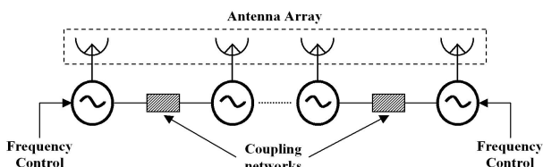
Fig. 1. Block Diagram of an array of N-coupled oscillators.
