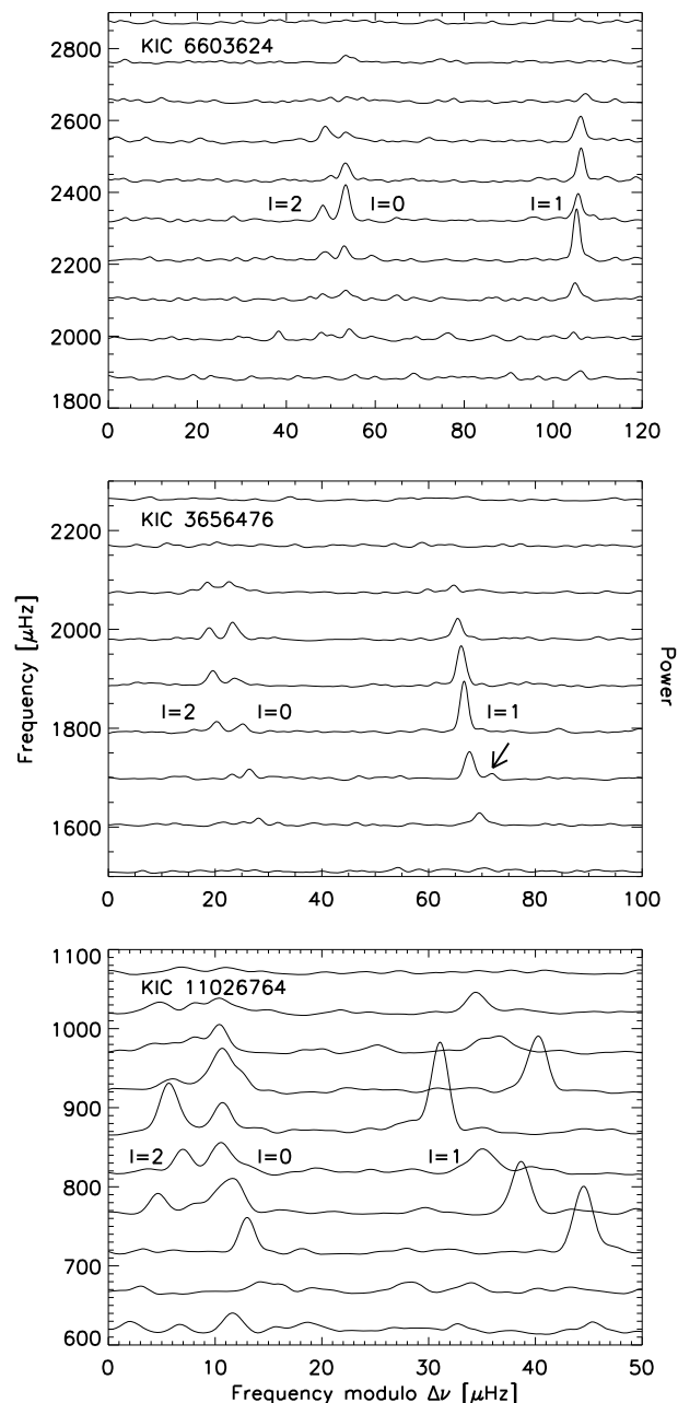
Fig. 3 Échelle diagrams of the three G-type stars analyzed by Chaplin et al. (2010). The spectra have been smoothed by a Gaussian running-mean with a width of 2 \mu\text{Hz} , before substrings of the spectra were stacked on top of one another. The large separation in the three stars were measured to 110.2 \pm 0.6 , 94.1 \pm 0.6 and 50.8 \pm 0.3 \mu\text{Hz} (from top to bottom).
