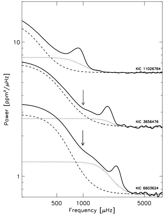
Fig. 2 Power density spectra of the three G-type stars analyzed by Chaplin et al. (2010), smoothed by Gaussian running-means of width of two times the large frequency separations. The spectra of KIC 3656476 and KIC 11026764 have been shifted upwards by 1 and 5 \text{ppm}^2/\mu\text{Hz} , respectively. The arrows mark the locations of the signature of faculae. The dashed and dotted lines show the best-fitting models of the granulation and facular components, respectively.
