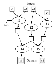
Fig. 2. Instance of a data-flow graph associated to the execution of five tasks \{f_1, \dots, f_5\} . The input parameters of the program are \{e_1, \dots, e_4\} whereas the outputs (i.e the results of the computation) are \{s_1, s_2\}
