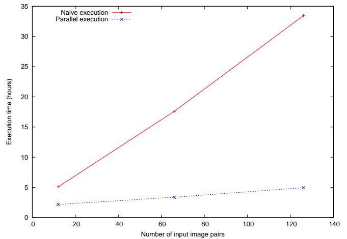
Figure 7. Execution performances
