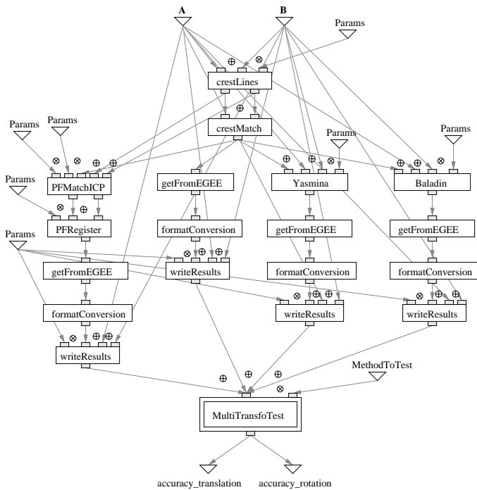
Figure 6. Application workflow
