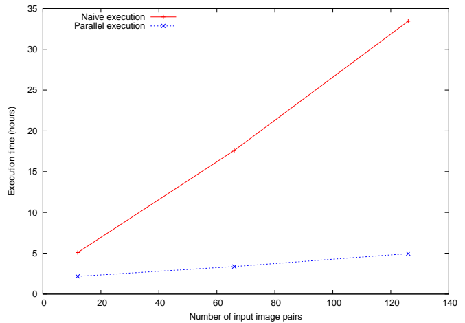
Figure 7. Execution performances
