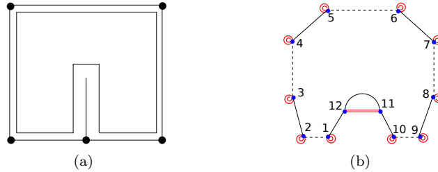
Figure 19: (a) an object where an edge is bended onto itself. (b) corresponding 2-gmap.
