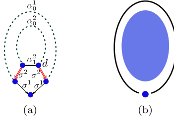
Figure 14: (a) A chain of maps encoding a 2d -disk, where dart d satisfies \langle \alpha_0^2 \rangle (d) = \langle \alpha_0^2 \rangle (d\alpha_1^1) . (b) The corresponding cellular subdivision.
