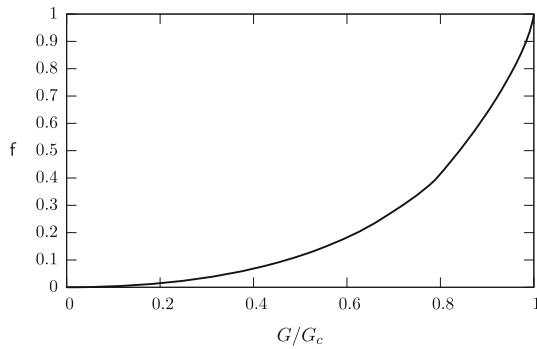
Fig. 8 Graph of the function f giving the fatigue law
