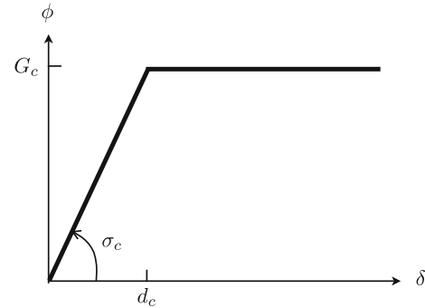
Fig. 2 Dugdale’s surface energy density
