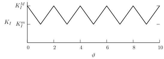
Fig. 9 Non simple cyclic loading: the rescaled stress intensity factor K_I oscillates between K_I^m and K_I^M (the true one K_I = \sqrt{\epsilon}K_I )
