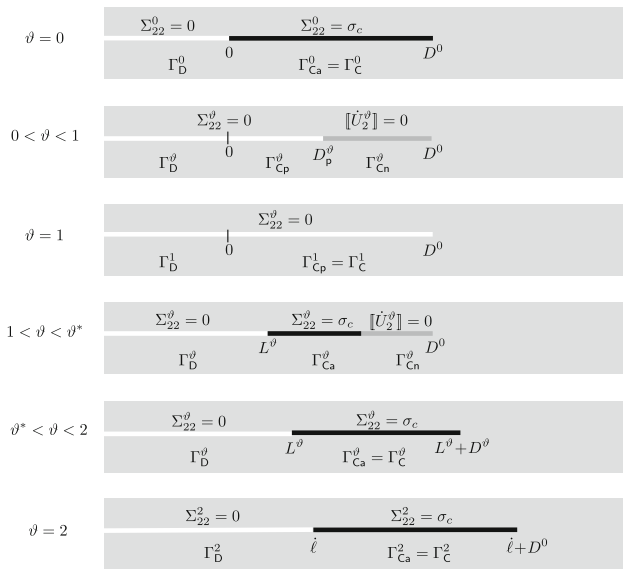
Fig. 4 Evolution of the non cohesive crack and of the cohesive crack during a cycle: in white, the non cohesive crack or the passive part of the cohesive crack; in gray, the neutral part of the cohesive crack; in black, the active part of the cohesive crack. The associated boundary conditions in terms of the normal stress or of the opening rate are indicated. The main stages of the evolution are as follows: at \vartheta = 0 , all the cohesive crack is active and the cohesive stress is equal to \sigma_c ; during the unloading phase, 0 < \vartheta < 1 , the cohesive crack becomes progressively passive, the cohesive stress is equal to 0 in the passive part while the opening does not evolve in the neutral part; at \vartheta = 1 which corresponds to the end of the unloading phase, all the cohesive crack is passive; during the first part of the loading phase, 1 < \vartheta < \vartheta^* , the tip of the non cohesive crack propagates while the tip of the cohesive crack does not evolve, a part of the cohesive crack remains neutral, the cohesive stress is equal to \sigma_c in the active part while the opening does not evolve in the neutral part; at \vartheta = \vartheta^* , all the cohesive crack is active; during the second part of the loading phase, \vartheta^* < \vartheta < 2 , all the cohesive crack is active, both the tip of the cohesive crack and the tip of the non cohesive crack propagate; at \vartheta = 2 , the tip of the non active crack is at \dot{\ell} and the length of the cohesive crack is D^0 again
