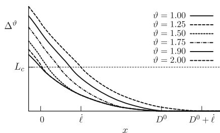
Fig. 6 Evolution of the cumulated opening and of the different zones (non cohesive zone, active zone and process zone) during the loading phase of a cycle when G/G_c \approx 0.636 (then \hat{\ell} = D^0/3 ). Note the two
