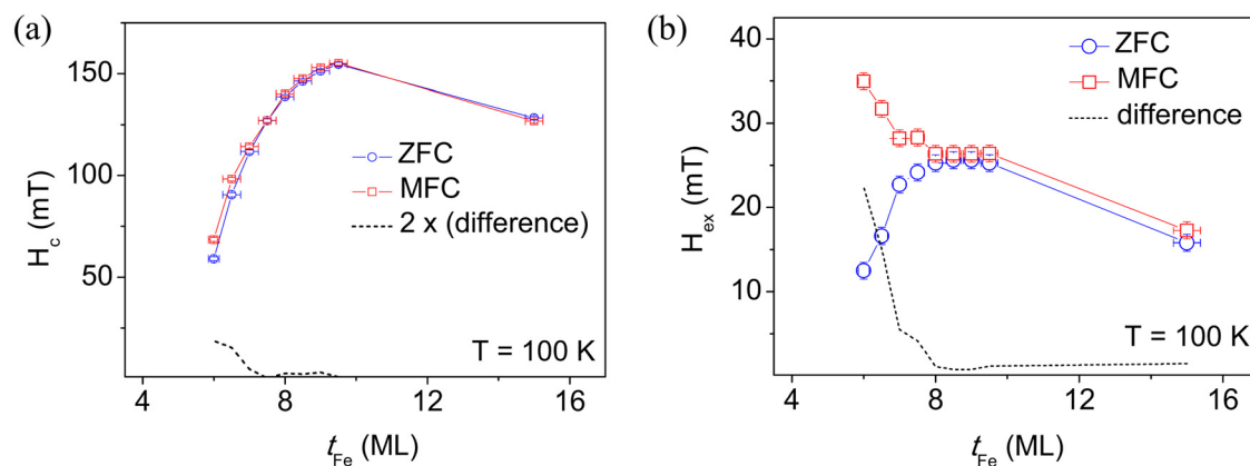
FIG. 2. (Color online) Dependence of (a) coercivity ( H_c ) and (b) exchange bias ( H_{ex} ) on the nominal Fe thickness ( t_{Fe} ). The values were extracted from hysteresis loops measured after zero field cooling, ZFC (circles) and magnetic field cooling, MFC (squares) and warming to 100 K. Dotted line in (a) shows two times the difference between the coercivities for MFC and ZFC.
