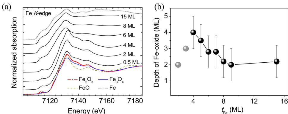
FIG. 4. (Color online) (a) XANES at the Fe K -edge for various thicknesses of Fe (solid lines). Also shown are the reference spectra for the \text{Fe}_2\text{O}_3 , \text{Fe}_3\text{O}_4 , \text{FeO} and Fe phases for comparison and, (b) the estimated depth of the Fe-oxide, t_{\text{ox}} , plotted against the nominal Fe thickness, t_{\text{Fe}} . Grey dots indicate that the whole depth of Fe was oxidized ( t_{\text{ox}} = t_{\text{Fe}} ).
