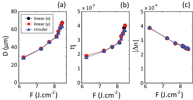
FIG. 3. Diameter D of the thermally affected zone (a), spin-to-orbital angular momentum conversion efficiency \eta (b) and the estimated radial birefringence \Delta n (c) [see text for details] as a function of the fluence. Data are shown for different polarization states of the writing beam as indicated in panel (a).
