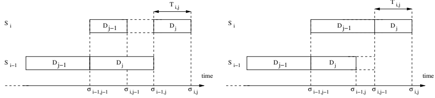
Fig. 18.4: Two different configurations for an execution with service parallelism but no data parallelism.
