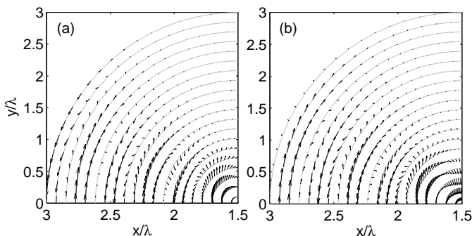
Fig. 11: Vector representation of the normalized electric field \mathbf{E}[\mathbf{E}_{\text{TR}}(\mathbf{r}, \omega)]/G(r) shown in Fig. 10: (a) real and (b) imaginary part. As the wavefront closes onto the focal region, the electric field passes from the TEM configuration typical of far-field radiation to a \hat{\mathbf{y}} -oriented configuration, reminiscent of the original field distribution of the synthetic aperture.
