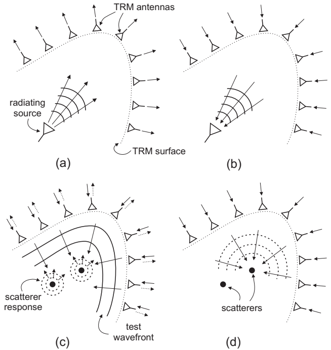
Fig. 1: A schematic representation of the two main TR techniques currently available: (a)-(b) TR of a radiating source; (c)-(d) selecting focusing over a point scatterer by means of the DORT approach.
