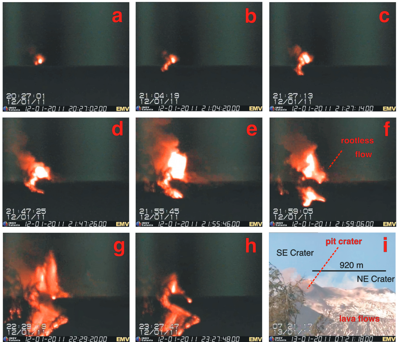
Figure 3. Visible images collected from EMV and giving a view from the east, over a 11 km distance, of the eruption site. (a) The brightest spot represents the Strombolian activity from the pit crater on the east flank of the SE Crater, the smaller spot on the left being the lava flow from the lower rim of the pit crater. (b) Strombolian activity increases, and the lava flow spreads SE. (c) Low lava fountaining starts, with a small ash plume dispersed SE (left) and lava flow extending down the upper Valle del Bove. (d–g) Lava fountaining increases in intensity and lava flow field grows. (h) Decreasing explosive phase and declining lava output. (i) Daytime view on 13 January, showing red ash emission from the pit crater, and the inactive lava flow field in the upper Valle del Bove is clearly visible, although partially obscured to the left by a tree. Date and time formats are as in Figure 2.
