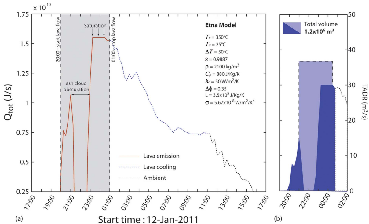
Figure 12. Power flux extracted from SEVIRI data showing the trends associated with lava emission, plume obscuration, saturation, and cooling. During the effusive phase power flux was converted to TADR using model parameters given [see Gouhier et al. , 2011]. In addition the cooling curve was used to estimate the total volume of erupted lava, allowing us to reconstruct the TADR curve as given at the right. For the TADR curve, TADRs calculated using unsaturated, cloud-free data are given by dark tones, and the “missing” volume obtained from the cooling curve is given by the light tones.
