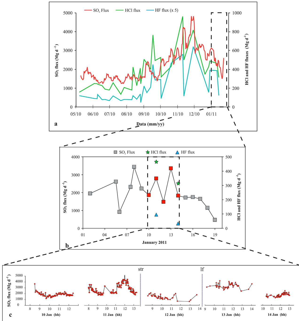
Figure 7. (a) Long-term variations in the 7-point-running mean SO 2 flux (red line; primary y axis) and discrete HCl and HF flux measurements (green and light blue lines, respectively; secondary y axis). Note that, to plot HF flux on the y axis, we have multiplied it by five. (b) Daily averaged SO 2 flux measured by the Flame network between 2 and 19 January 2011, together with the HCl (green stars) and HF (light blue triangles) fluxes measured on 11 and 14 January. (c) Magnified time-window showing the daytime SO 2 flux measured between 10 and 14 January 2011. Dotted-blue lines indicate the onset of the Strombolian (str) and lava fountain (lf) activity.
