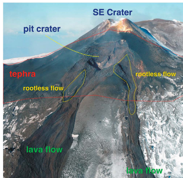
Figure 11. Photo taken from the east during a 14 January 2011 overflight showing the depression on the east flank of the SE-Crater (pit crater) which was the source of explosive and effusive activity on 11–13 January 2011. Volcanic ash dispersal covering the snow toward the south (left in the picture) does not cover the summit of the SE-Crater, thus showing that this crater did not produce any explosive activity during the eruptive episode. Note the two lava flows extending from the depression on the east flank of the SEC toward the Valle del Bove, which were emplaced during the night of 12–13 January. The two rootless flows produced by the remobilization of tephra have been marked using a yellow dotted line. Photo courtesy of Alfio Amantia.
