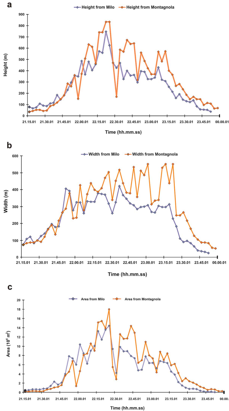
Figure 9. Graph of the (a) height, (b) width, and (c) area of the lava fountains calculated from the images of EMV (Milo) and EMOT (La Montagnola) against time during the fountaining episode of 12–13 January 2011.
