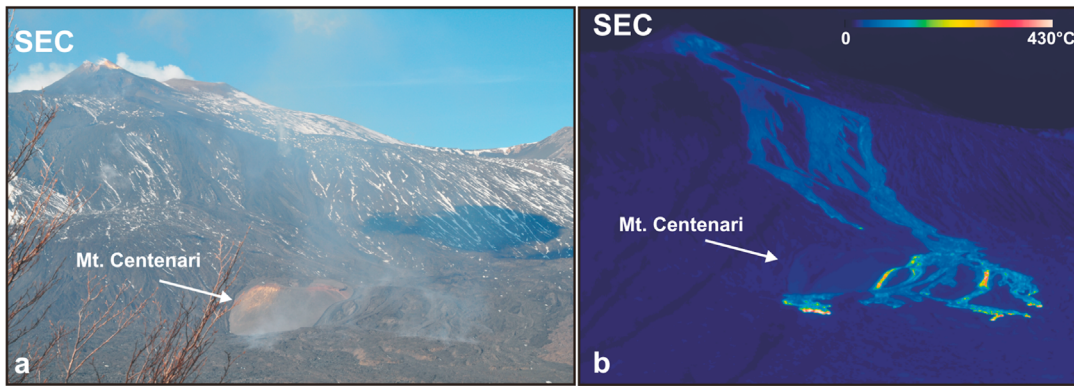
Figure 10. (a) Photo and (b) corresponding thermal image of the lava flow field emplaced in the Valle del Bove on 12–13 January 2011, taken from SE. Both images show that the lava flow field is cooling. The high temperature areas of the lava flow field relate to the front widening on Valle del Bove floor and to still moving lava due to channel drainage. Photograph in Figure 10a is courtesy of Stefano Branca.
