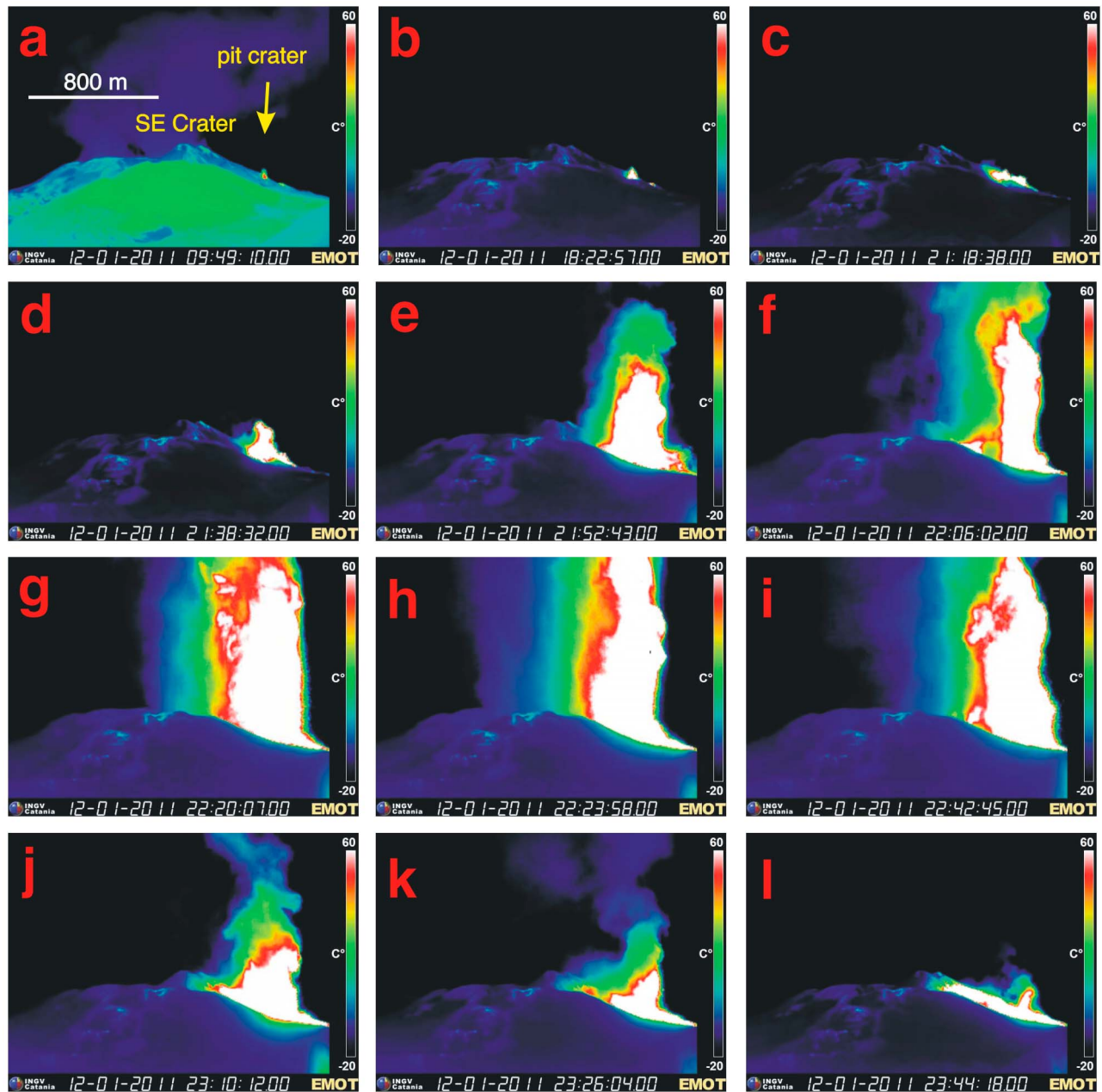
Figure 2. (a–l) Thermal images recorded from EMOT (see Figure 1). The saturated portion of the eruptive vent and lava fountain is displayed in white. On the black line below each image we give the date (dd-mm-yyyy) and UTC time (hh:mm:ss:00). Note the eastward (right) shift of the vent as apparent by comparing Figures 2b and 2l, and which occurred between Figures 2e (21:52:43) and 2f (22:06:02).
