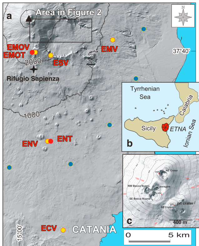
Figure 1. (a) Map of the SE flank of Etna [modified after Behncke et al. , 2009] showing the location of the INGV-CT thermal (red circles) and visible (yellow circles) camera stations (see Table 1 for details). Blue circles indicate the position of UV-scanner stations of the FLAME network. Labels are as follows: EMOT, EMOV = thermal and visible cameras located at La Montagnola; ESV = visible camera located at Schiena dell'Asino; EMV = visible camera located at Milo; ENT, ENV = thermal and visible cameras located at Nicolosi; ECV = visible camera located at CUAD. The black triangle indicates the position of the summit craters (magnified in Figure 1b), and the rectangle is the area effected by the 11–13 January 2011 eruption and represented in Figure 6. (b) Map of southern Italy, showing the position of Sicily and Mount Etna. (c) The summit craters of Mount Etna [modified after Neri et al. , 2008]. Labels are as follows: NEC = NE-Crater; VOR = Voragine; NW BN: NW pit of Bocca Nuova; SE BN: SE pit of Bocca Nuova; SEC: SE-Crater.
