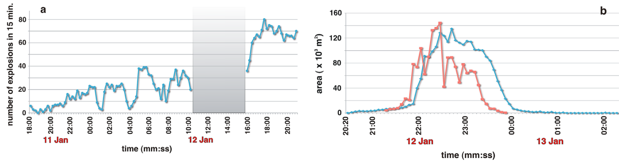
Figure 5. (a) Number of explosions occurring in 15 min time windows during 11–12 January 2011. The gray shaded area lacks data due to clouds obscuring the summit. (b) Time evolution of active lava flow area (blue line) and lava fountain area (red line), as seen from EMV.
