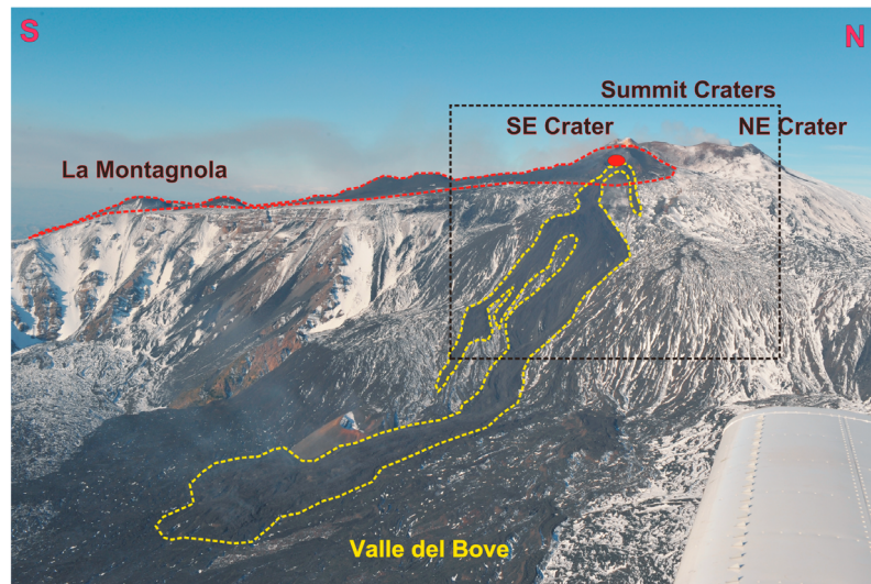
Figure 6. Photo of the 12–13 January 2011 lava flow field taken from the east during an airplane survey on 13 January. The yellow dotted line marks the boundary of the lava flow field, and the red dotted line shows the SSW dispersed ash erupted during the lava fountaining episode. The red circle displays the location of the pit crater on the eastern flank of the SEC that gave rise to the 11–13 January eruptive activity, and the black dotted square shows the area framed by EMV and displayed in Figure 3. La Montagnola is the location of EMOT and EMOV cameras (~3 km from the SEC, see Figure 1). Photo courtesy of Alfio Amantia.
