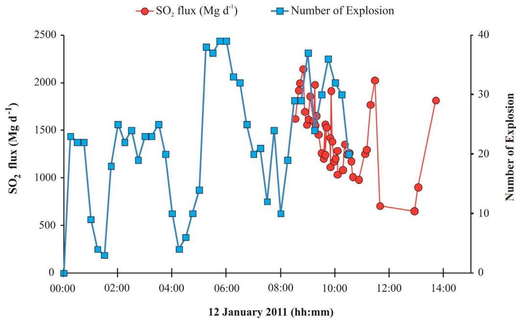
Figure 8. Number of explosions and daytime SO 2 flux recorded on 12 January 2011.
