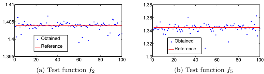
Fig. 1: Estimated minimax values for 100 initializations, compared to reference
