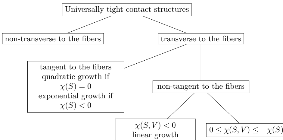
FIGURE 1. Universally tight contact structures on circle bundles over a surface S of non-positive Euler characteristic.
