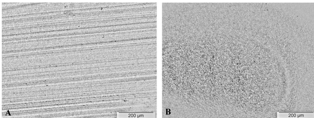
Figure 14: Light microscopic images of PCL composites with different CNT contents; A: 0.5 wt.%, B: 1.0 wt.%
