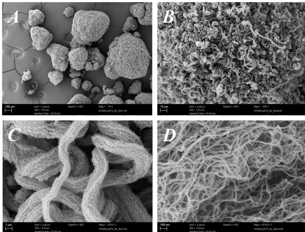
Figure 4: SEM micrographs of CNT N7000 raw material at different magnifications
