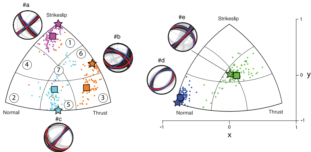
Figure 10. The results of the first synthetic resolution test. For each event, the stereodiameter displays the expected fault plane solution (blue), the recovered fault plane solution (red), the 'perturbed fault plane solutions' inside the confidence interval (eq. 1) (black) and the 'perturbed fault plane solutions' outside the confidence interval (grey). The ternary diagrams display for each event the solution to retrieve (star), the recovered solution (square) and the 'perturbed solutions' (dot). Each corner of the triangle corresponds to the vertical null-axis (strike-slip fault), P -axis (normal fault) and T -axis (thrust fault). The line inside the ternary diagram indicates the 30^\circ plunge angle of the null-, P - and T -axis and delineates seven areas corresponding to a type of focal mechanism: strike-slip fault (Area 1), normal fault (Area 2), inverse fault (Area 3), normal-strike-slip fault (Area 4), dip-slip fault (Area 5), thrust-strike-slip fault (Area 6) and mixed fault (Area 7).
