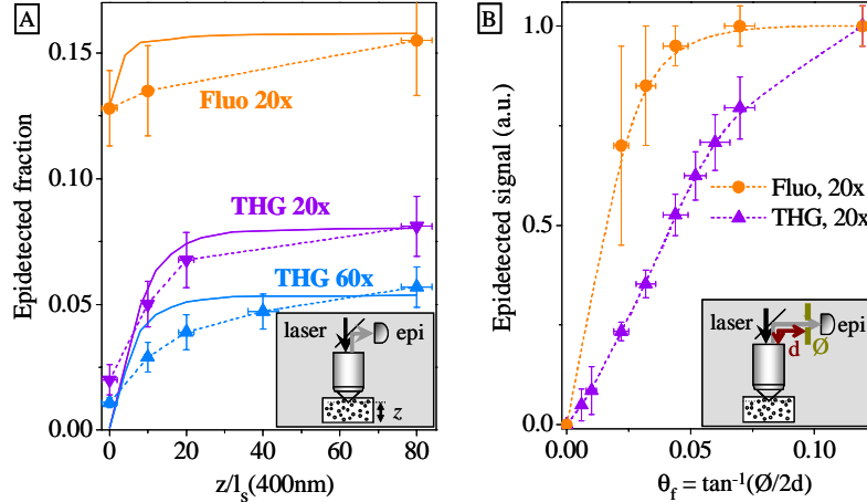
Fig. 7. Incidence of the microscope angular acceptance (field of view) on epidetection of THG and 2PEF from a turbid medium. (A) Measured epidetected fraction as a function of slab thickness (symbols and dotted lines), and corresponding Monte Carlo simulations (plain lines) for two different objectives (60 \times , 0.9NA and 20 \times , 0.95NA). Simulations assume that l_s^{(400)}=25\mu\text{m} and that the angular field of view is clipped to 0.13 rad (half-angle) by the collection optics. (B) Measured epidetected THG and 2PEF signal at the center of the field, as a function of the angular acceptance of the collection optics.
