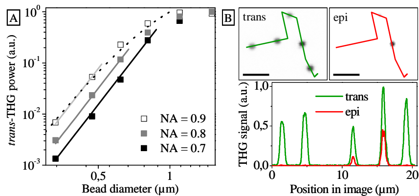
Fig. 5. Visibility of dielectric and metallic particles in THG microscopy. (A) Sixth-power dependence of the trans-THG signal on dielectric bead size. Squares: signal obtained from the center of individual polystyrene beads embedded in agarose and centered at the beam focus. Plain lines: sixth-power fits. Dotted line: numerical calculation for NA=0.9 and linear indexes of polystyrene (1.57 at 1180 nm and 1.61 at 393 nm). (B) Top: trans- and epi-detected THG images of a transparent gel containing 330-nm polystyrene beads and 150-nm gold particles. Gold particles are visible in the epi image, whereas polystyrene spheres are not. Bottom: profile through the broken lines indicated in the images. Scale bar is 3 μm. Excitation wavelength is 1180 nm.
