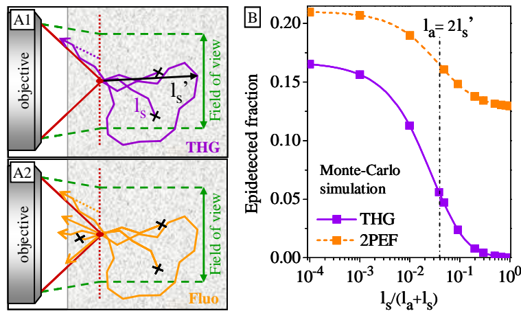
Fig. 6. Incidence of absorption and scattering on epidetection of backscattered harmonic light and multiphoton-excited fluorescence from a turbid medium. (A1) Detection of backscattered forward-emitted light (THG). (A2) Detection of light from an isotropic source (2PEF). (B) Epidetected fraction of THG and 2PEF as a function of tissue albedo ( g=0.92 , l_s=25\mu\text{m} , NA=0.95 , field of view= 1000\mu\text{m} , working distance= 2\text{mm} , sample thickness= 2500\mu\text{m} ).
