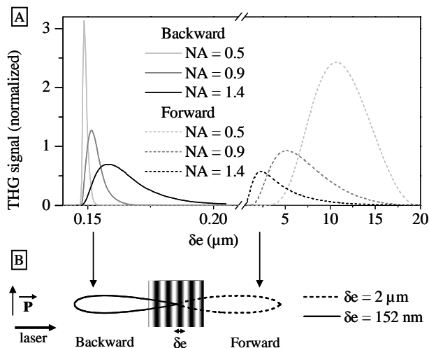
Fig. 4. Forward and backward emitted TH powers from an axially periodic (sine-like) object in a focused Gaussian beam, as a function of the spatial period \delta e . (A) Forward and backward emission for several NAs. (B) Radiation patterns for periodicities \delta e=2\mu\text{m} and \delta e=152\text{nm} (NA=0.9).
