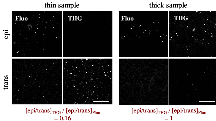
Fig. 8. Trans- and epi-detection of endogenous THG and multiphoton-excited fluorescence from a washed fresh lung tissue sample. Epi-THG imaging is possible only in thick areas, as opposed to epi-fluorescence. Epi/Trans image pairs were acquired simultaneously. THG and fluorescence images were recorded at different locations. Acquisition time, 10 \mu s/pixel. Scale bar, 50 \mu m.
