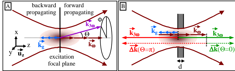
Fig. 1. (A) Geometry and notations (see text). (B) Wave vector mismatch in the forward and backward direction. A slab-like sample is shown for illustrative purpose (see discussion).
