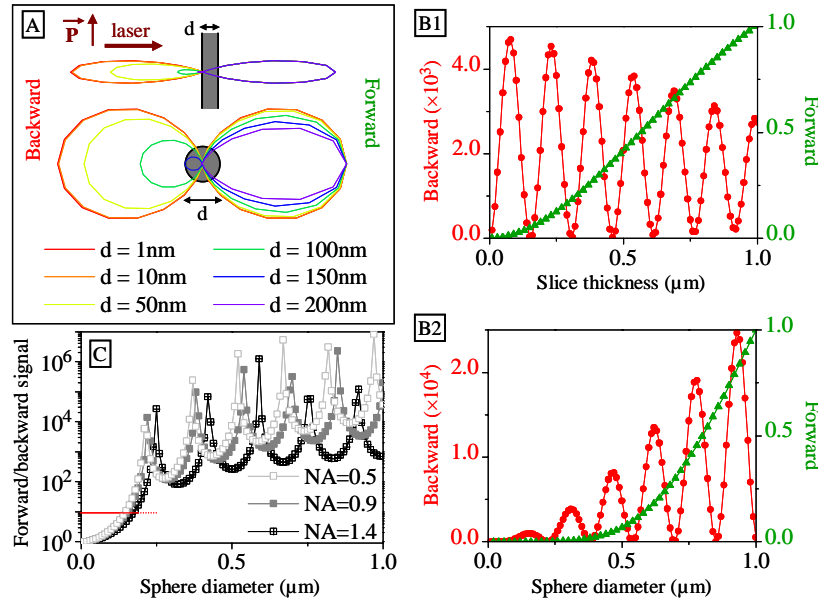
Fig. 3. TH emission patterns for a sphere and a thin slab at the focus of a Gaussian beam. (A) Normalized radiation patterns as a function of slab thickness (top) and sphere diameter (bottom). (B1) Slab: Forward (green triangles, right) and backward (red circles, left) emitted power as a function of thickness ( \text{NA}=0.9 ). (B2) Sphere: forward (green triangles, right) and backward (red circles, left) emitted power as a function of diameter ( \text{NA}=0.9 ). (C) Sphere: ratio of forward/backward emitted power as a function of diameter and excitation NA (semilog plot).
