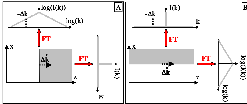
Fig. 2. Spatial frequency spectrum for an interface (A) perpendicular and (B) parallel to the excitation beam. In both cases, the large backward wave vector mismatch is not efficiently compensated by the sample structure.
