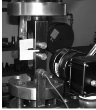
Fig. 9. Compact tension test specimen and DIC system.
