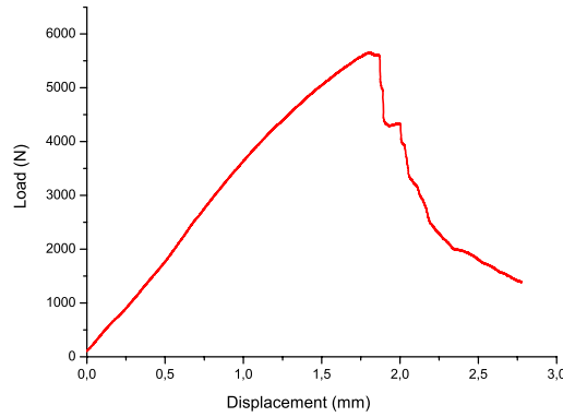
Fig. 14. Load-displacement in a CC test specimen.
