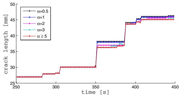
Fig. 3. Relation between the crack length and time for different values of \alpha .
