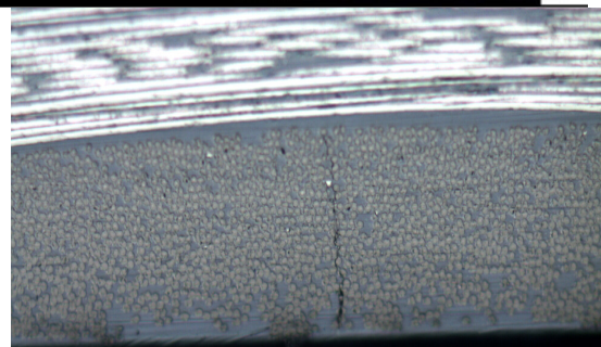
Damage location 3-1(Surface yarn) side view
